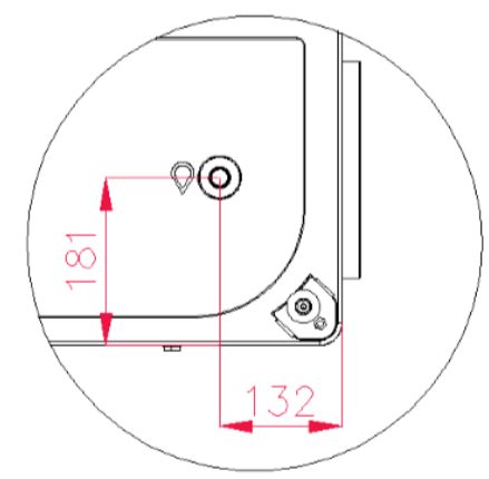
A - backview
